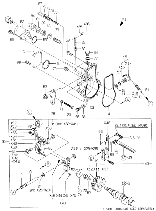
13. GOVERNOR
